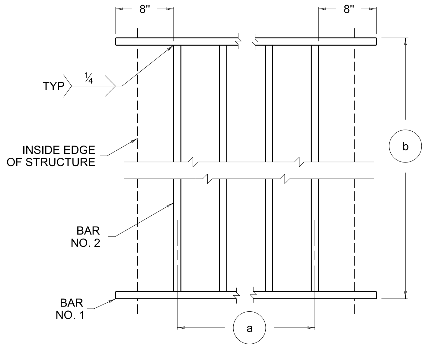
TYPICAL GRATE
